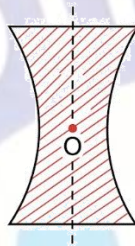
Concave lens
